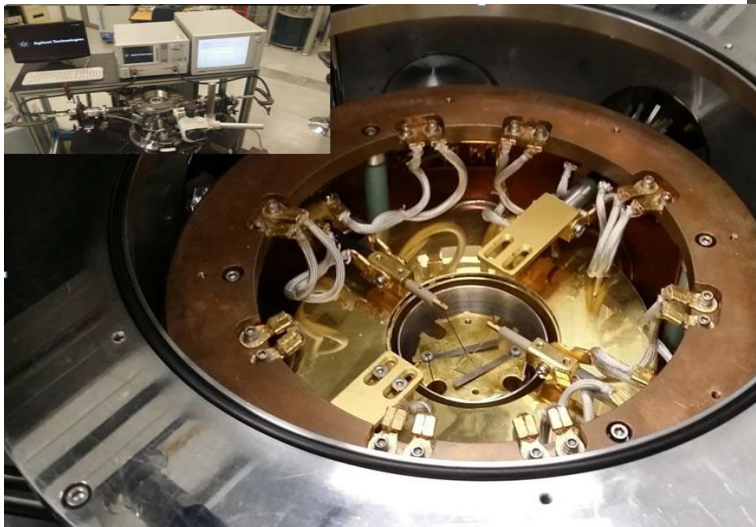
Diamond deposition chamber
