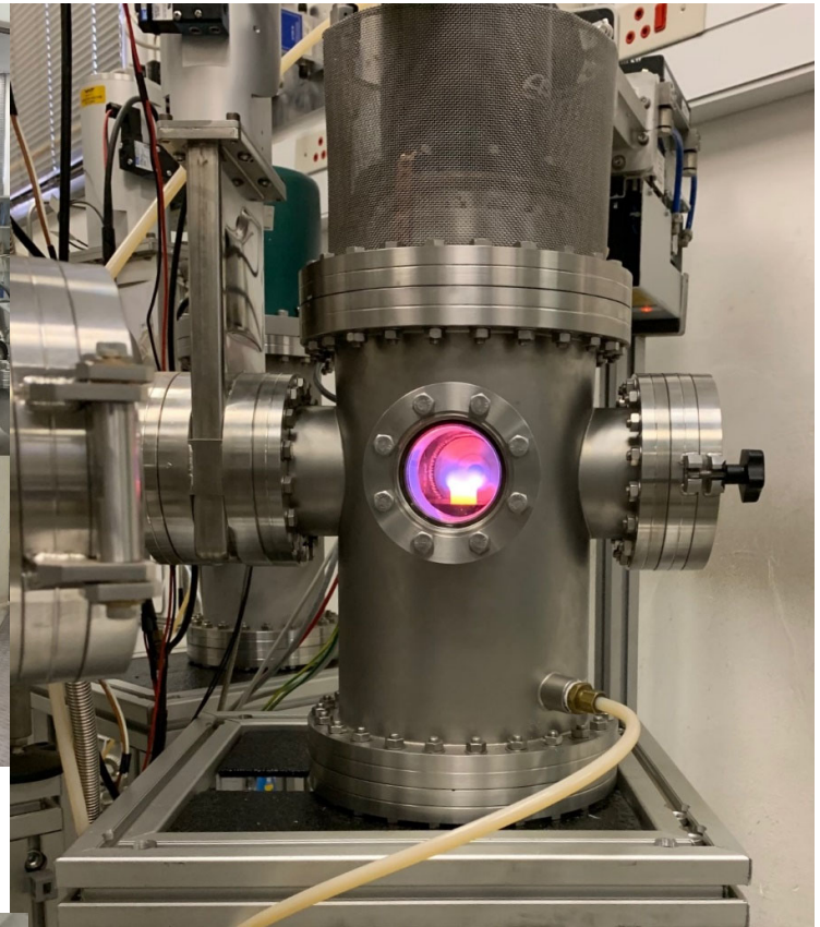
Diamond deposition chamber
